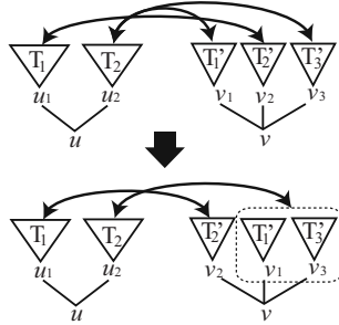
Fig. 2. Example for transformation to ordered trees
